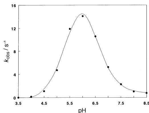
Fig. 7 pH Dependence of k_{\text{obs}} for the oxidation of \text{Mn}^{\text{II}}(\text{acac}) complexes by \text{ON}(\text{SO}_3)_2^{2-} . Experimental conditions: [\text{Mn}^{\text{II}}] = 1 \times 10^{-3} , [\text{ON}(\text{SO}_3)_2^{2-}] = 5 \times 10^{-5} , [\text{acac}] = 0.25 \text{ mol dm}^{-3} , T = 25^\circ\text{C} , I = \text{mol dm}^{-3}
