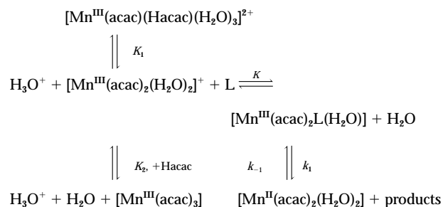
Scheme 3 L = \text{HONH}(\text{SO}_3)^- or \text{HON}(\text{SO}_3)_2^{2-}
